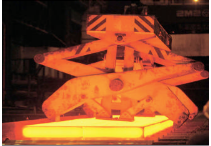
1200°C 25MT Hot Slab Tong
